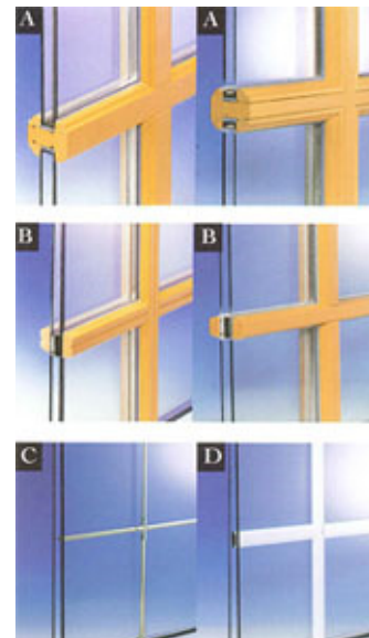
A - Glass divider bars B - Adhesive bars C - Brass bars D - Helima bars
